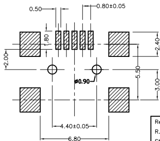
PCB LAYOUT TOLERANCES: ±0.05
